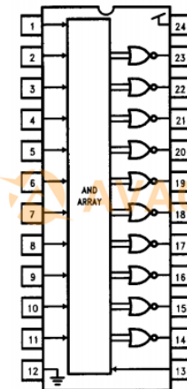
Block Diagram—PAL12L10
